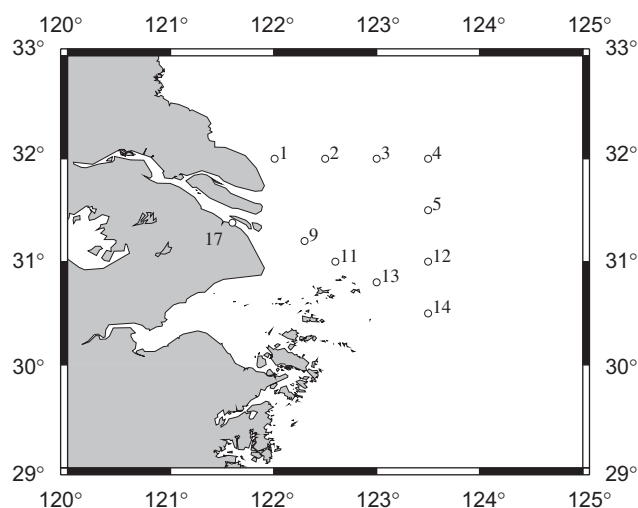
Fig. 1. Sampling stations off the Yangtze River estuary.
