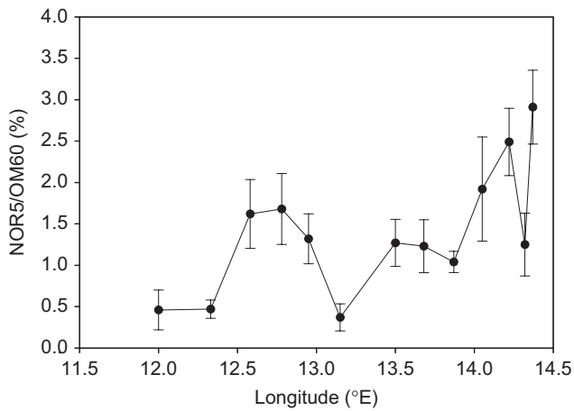
Fig. 5. NOR5/OM60 counts by CARD-FISH in the Namibian upwelling region on March 22–23, 2003, along 23°S near Walvis Bay. The counts were mostly at a depth of 10 m, with the exception of the two easternmost points that were at a depth of 15 m.
