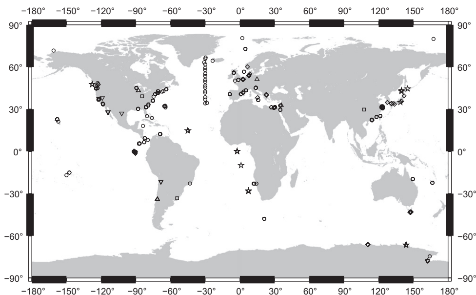
Fig. 3. Biogeography of the NOR5/OM60 clade. Sequence-, isolation-, and FISH-based identifications of NOR5/OM60 were marked on the world map. Signs refer to the habitat from where the sample was retrieved: marine water or other marine habitats – circle; marine coastal sediment – diamond; hypersaline – inverted triangle; soil – hexagon; fresh water – square; fresh sediment – triangle; deep sea – star. The map was created using the GMT (generic mapping tools) software package.
