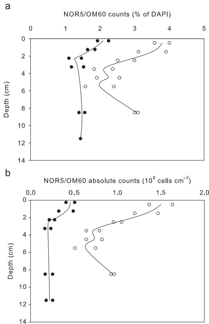
Fig. 6. NOR5/OM60 counts from Janssand sediment in March (black circles) and August (white circles) 2007. At each time point, two adjacent cores were sampled for duplication.
