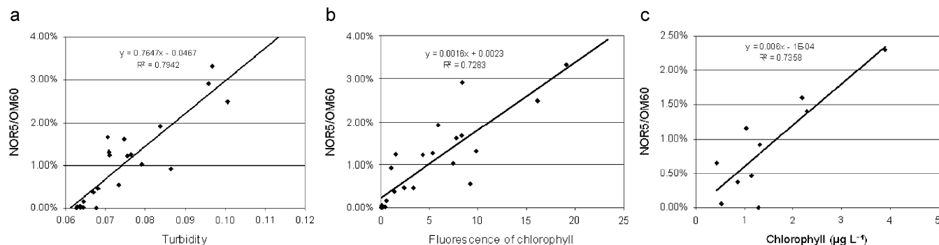
Fig. 7. Correlation of NOR5/OM60 to other environmental parameters: (a) turbidity in the Namibian transect, (b) chlorophyll fluorescence in the Namibian transect, (c) chlorophyll in the Yangtze River estuary.
