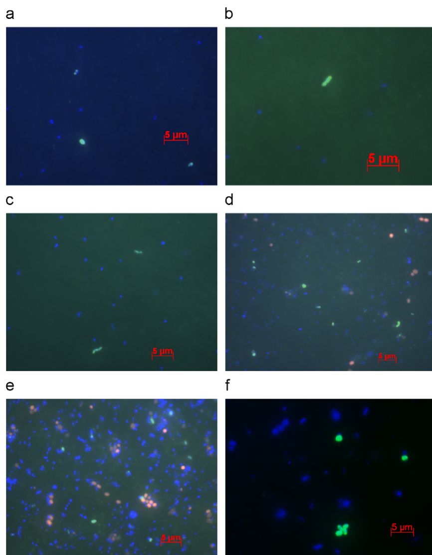
Fig. 4. Microscopic pictures of NOR5/OM60 cells in the environment: (a)–(c) North Atlantic open ocean, (d) and (e) from the Yangtze River estuary, (f) from Janssand sediment, North Sea. For all the pictures, blue: DAPI-stained DNA; green: fluorescein conferred probe signal for the NOR5/OM60 group; red: autofluorescence of cyanobacteria.
